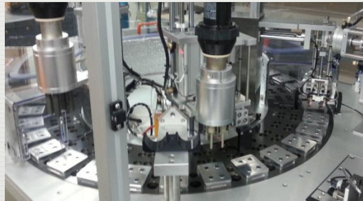
Lipstick filler(rotary)
